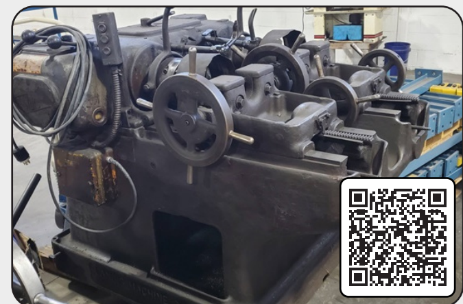
1" Landis Double Spindle Thread Cutter Ref. No. 26616
