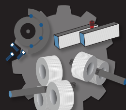
Thread Rolling
